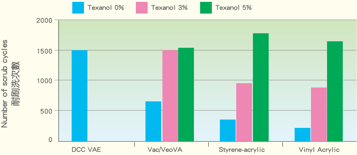
DCC VAE emulsion provides paint with good scrub resistance without the need of adding coalescing agent. 大連 VAE 乳液在無需添加成膜助劑的情況下也能賦予塗料優越的耐刷洗性能。
