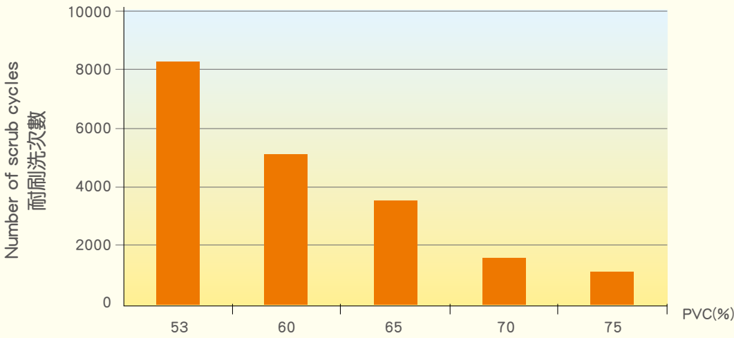
Paint formulated from DCC VAE emulsion shows excellent scrub resistance even at high PVC. 大連 VAE 乳液所製成的塗料在高 PVC 配方中依然擁有良好的耐刷洗性能。
